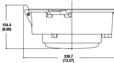
Driver Housing
